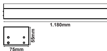
Dimension ( mm )
