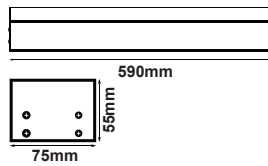
Dimension ( mm )
